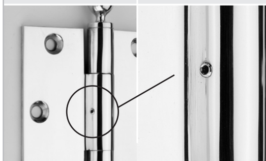
▲ Security Hinge (NRP) pin secured in place with stainless steel grub screw
